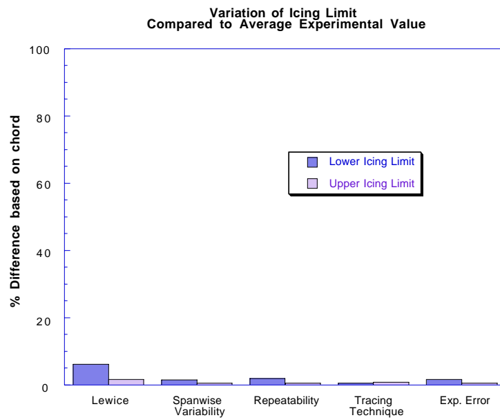
FIGURE 18. Variation of Icing Limit Compared to Average Experimental Value
